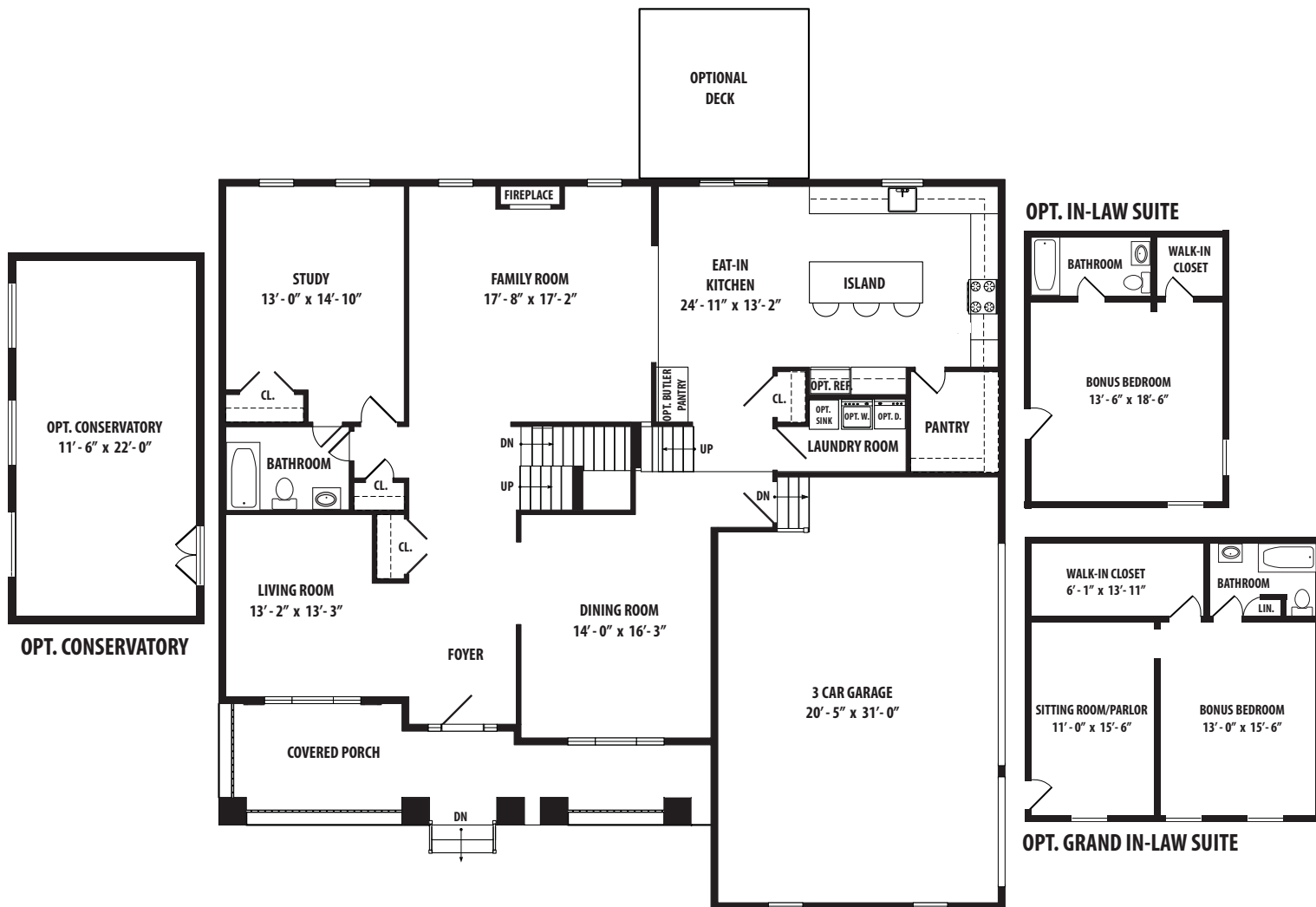
FIRST FLOOR
